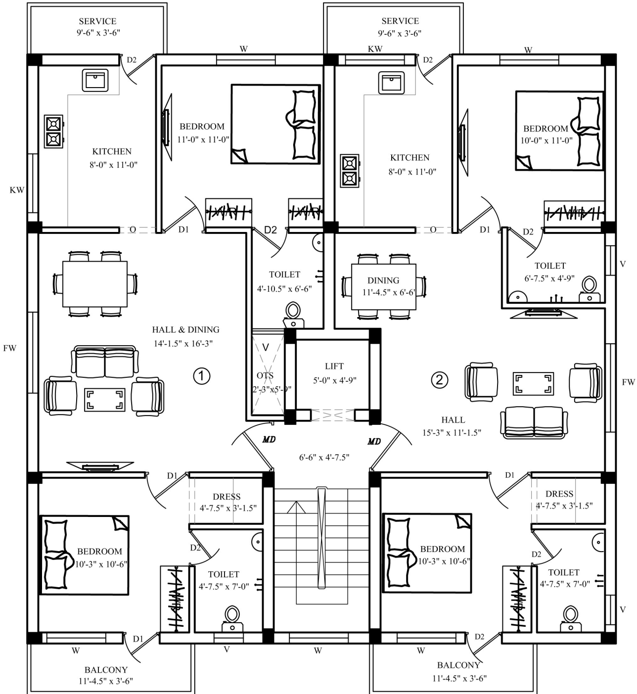
TYPICAL FLOOR PLAN (First, Second, Third)
